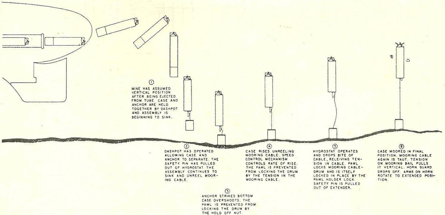
Planting sequence of mine Mk 10.
